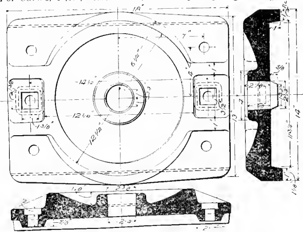
Figs. 4721-23. CAST-IRON TRUCK CENTER-PLATE.
